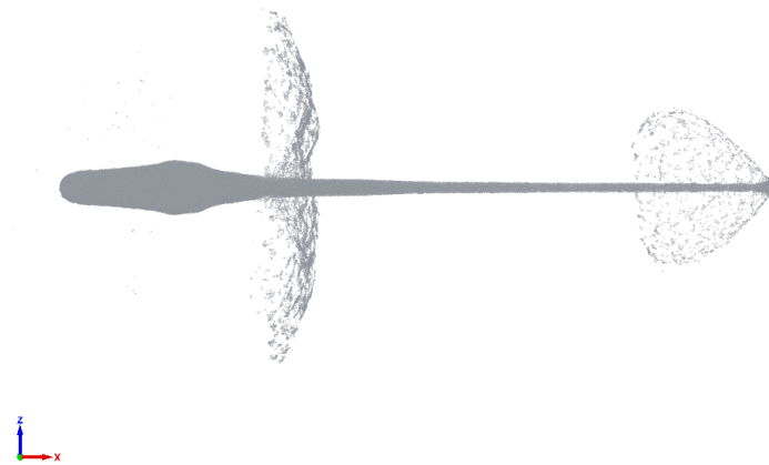
Figure 2. Shaped charge with full symmetry at final state.
