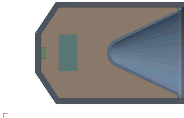
Figure 1. Shaped Charge at initiation, half symmetry.
