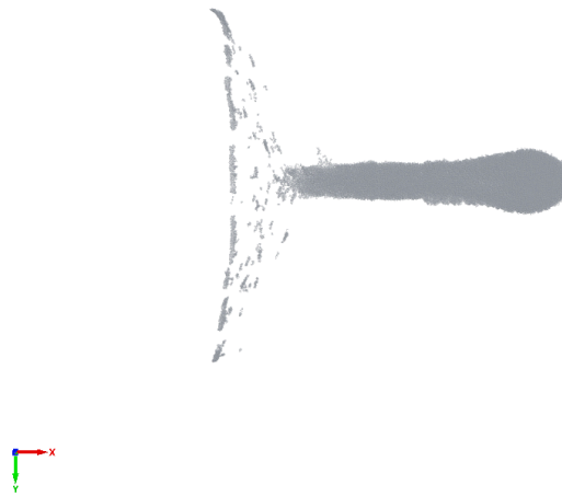
Figure 8. EFP with half symmetry at final state.
