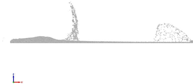
Figure 4. Shaped Charge with quarter symmetry at final state.
